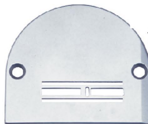
Needle plate (thread trimmer, light mat.) cod. 265 014728
