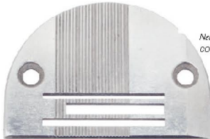
Needle plate (thread trimmer, very light mat.) cod. 212 010855
