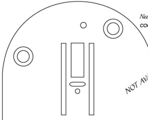
Needle plate cod. 199 001610
