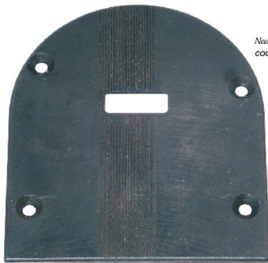
Needle plate mm. 8 (stitch L. 6 mm) cod. 367 205010
