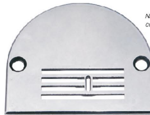
Needle plate (thread trimmer, medium mat.) cod. 265 005111
